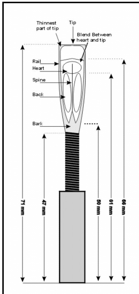
Figure 10 Oboe Reed Dimensions
