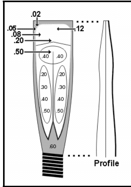
Figure 11 Measurements and Proper Profile
