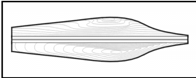
Figure 9 Oboe Reed Tip Profile
