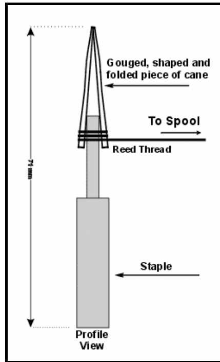
Figure 1 Reed Blank on Staple (side view)
